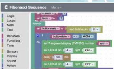
2. Block-based Programming
